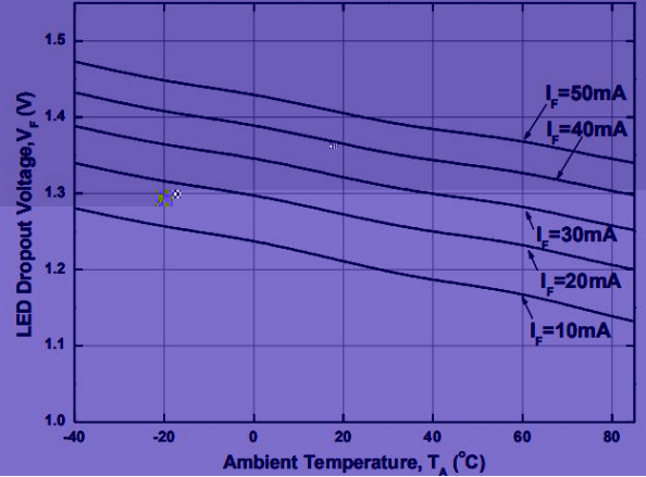
Figure 4. LED Dropout Voltage vs Ambient Temperature
