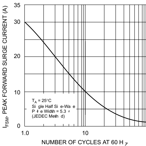
Fig. 3 Maximum Peak Forward Surge Current (e leg)
