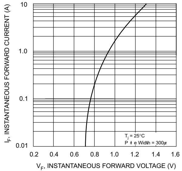
Fig. 2 Typical Forward Characteristic (e leg)
